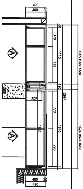
PLAN VIEW
