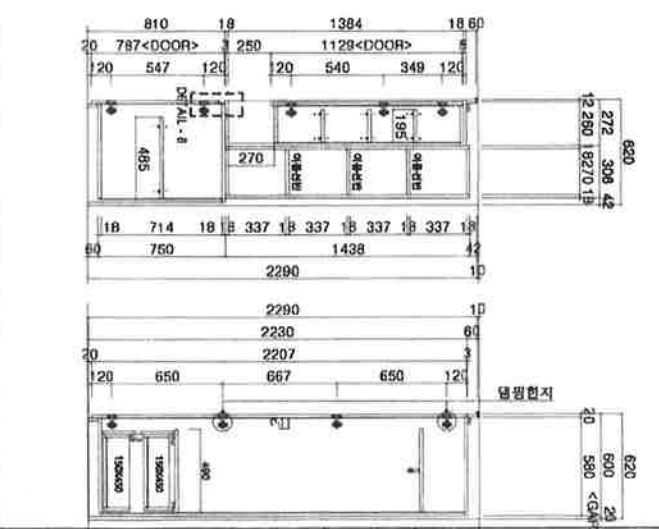
5 SECTION VIEW
