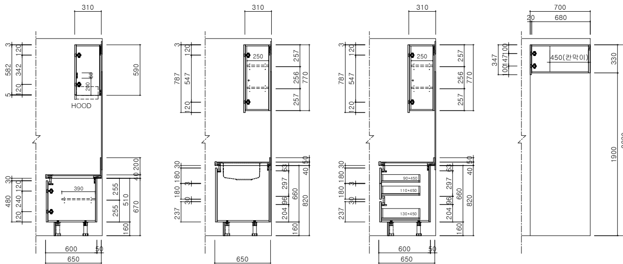
SIDE SECTION VIEW
