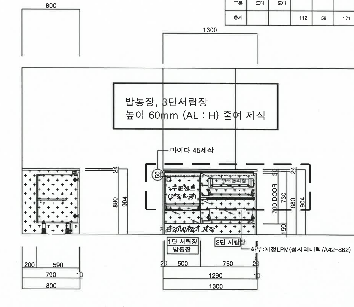
ELEVATION-C
