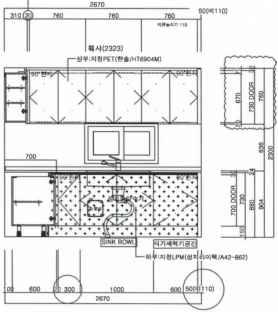
ELEVATION-B
