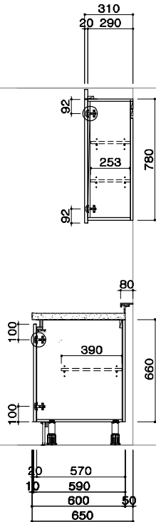
SIDE VIEW
