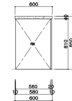
C ELEVATION
