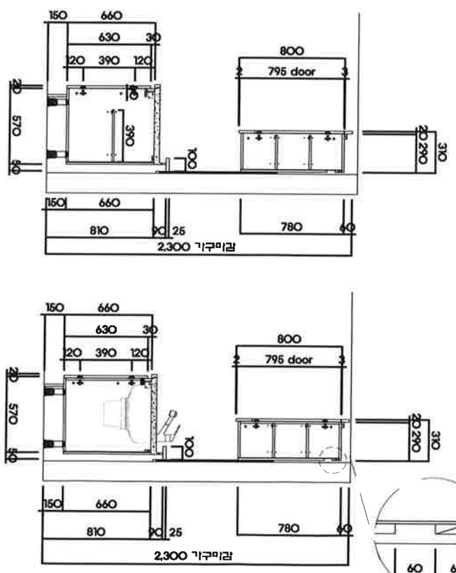
SIDE SECTION-A
