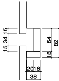
"A" DETAIL
