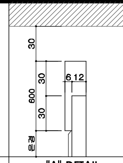
"A" DETAIL
