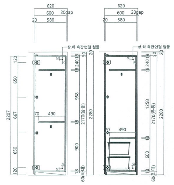
SIDE SECTION
