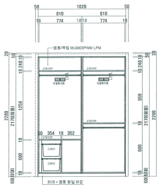
INNER VIEW
