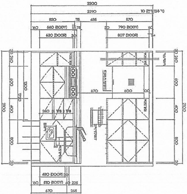
KITCHEN PLAN
