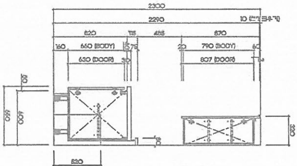
ELEVATION-B
