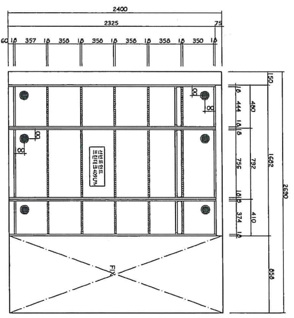
INNER VIEW
