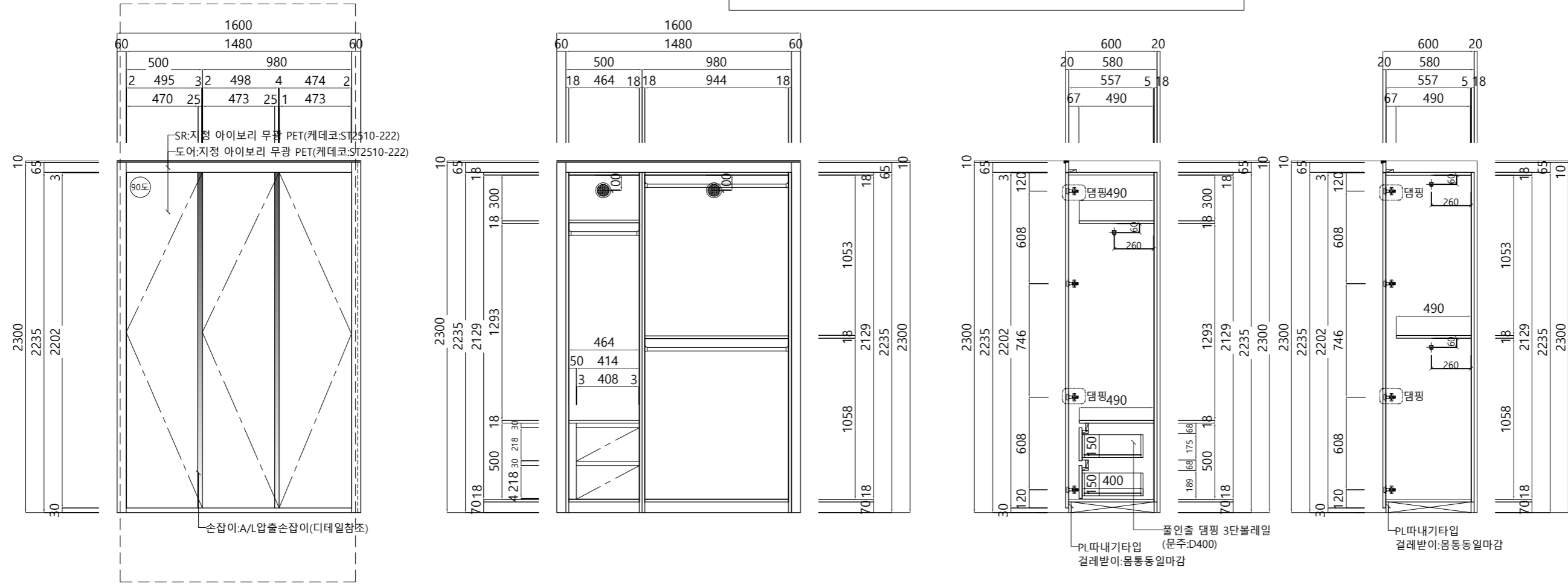
FRONT VIEW
