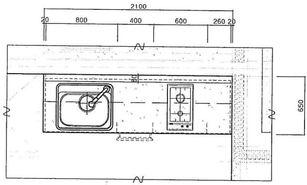
KITCHEN PLAN
