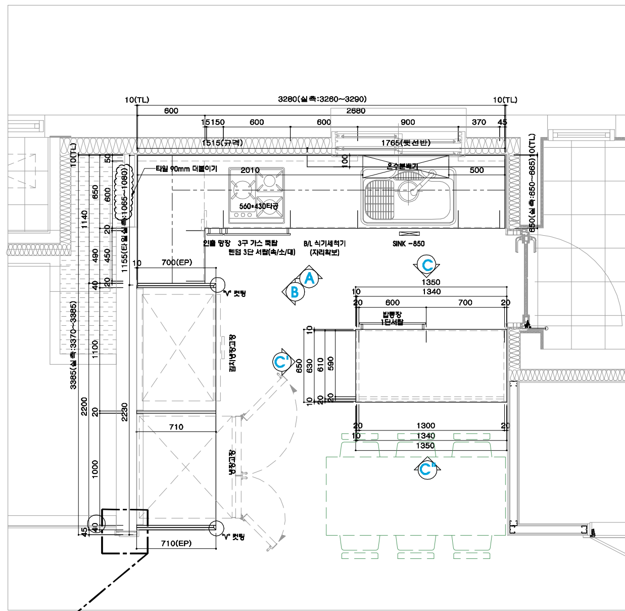
PLAN OF KITCHEN
