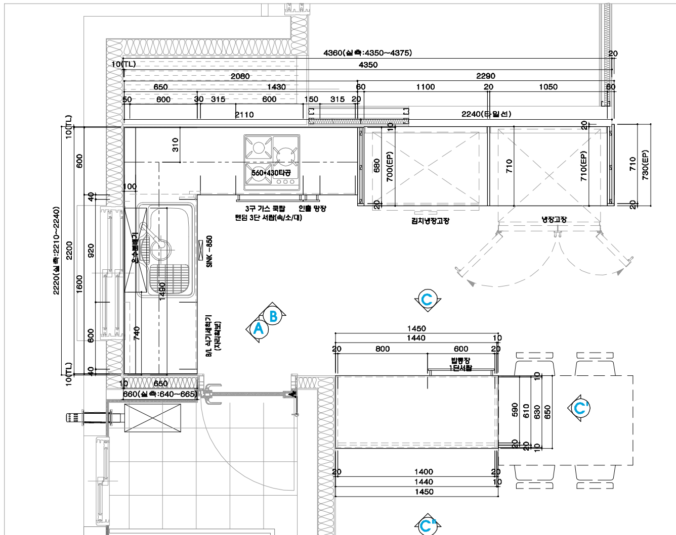
PLAN OF KITCHEN
