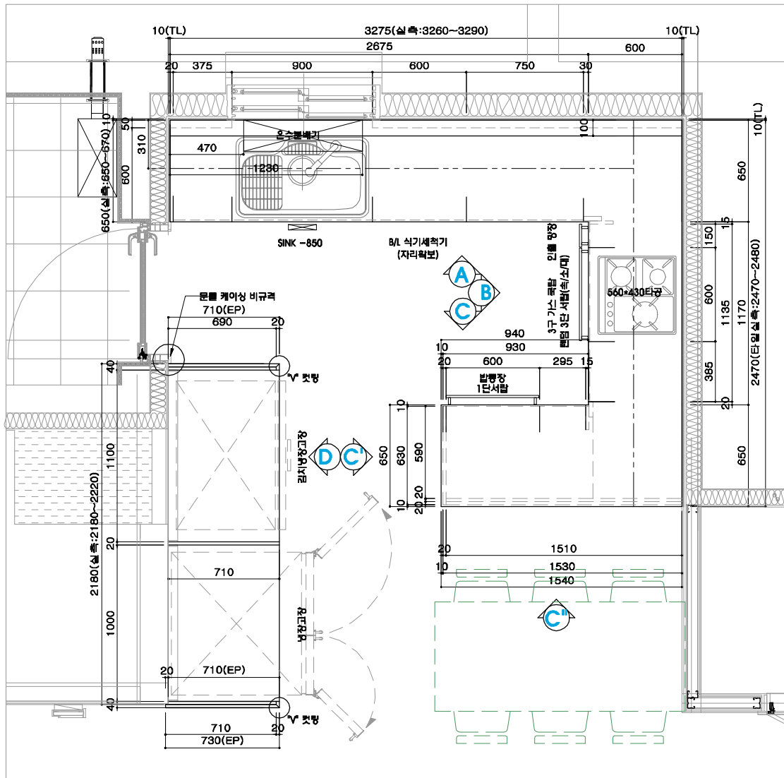
PLAN OF KITCHEN
