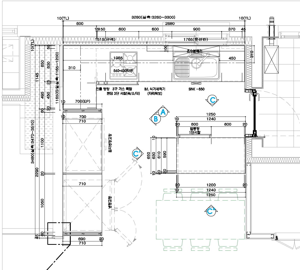
PLAN OF KITCHEN
