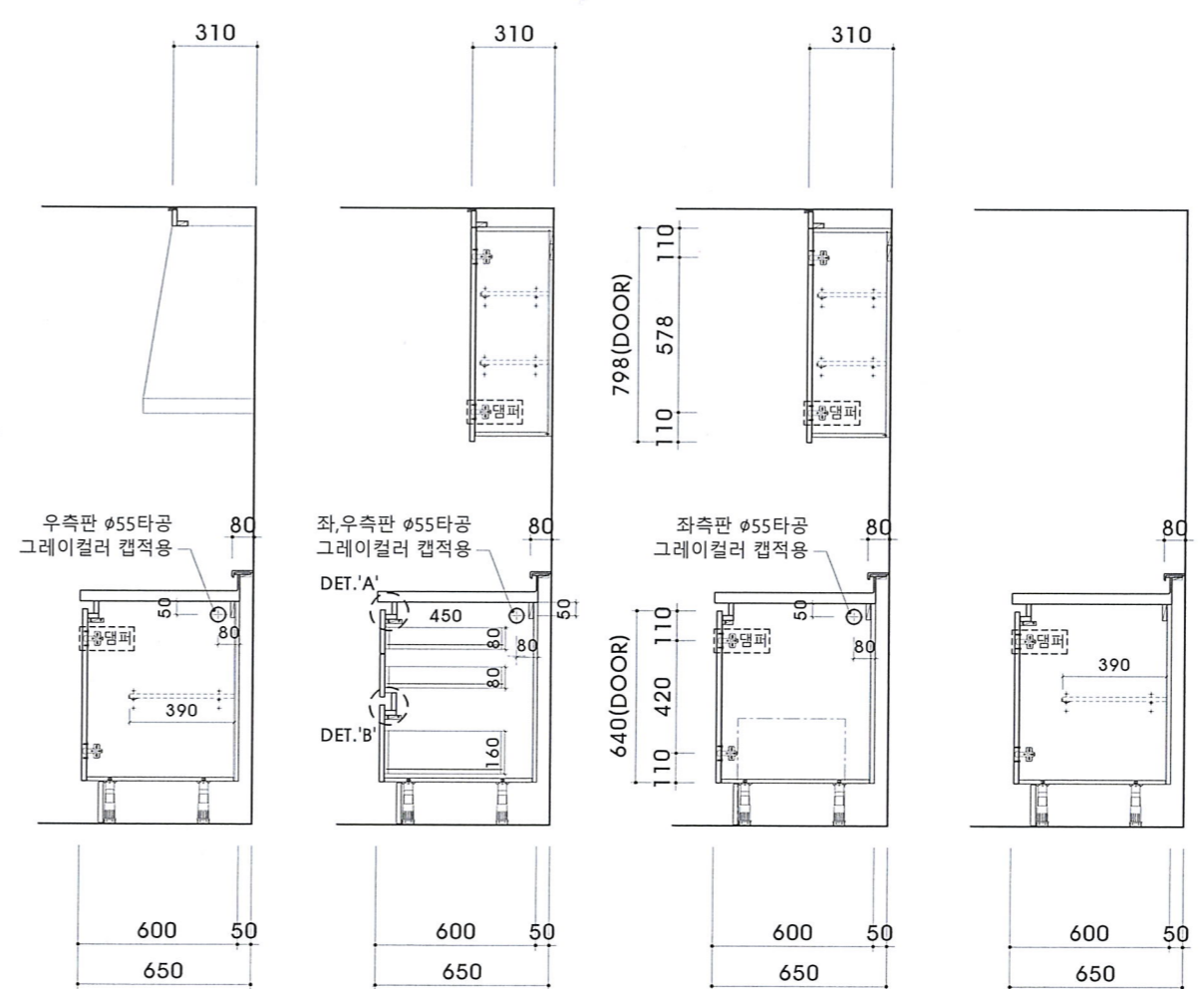
SIDE VIEW
