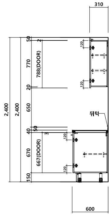
3 SECTION
