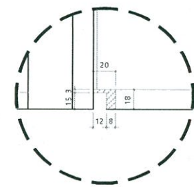
WALL UNIT GROOVE DETAIL
