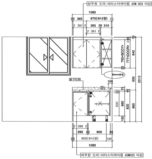
FRONT VIEW-A
