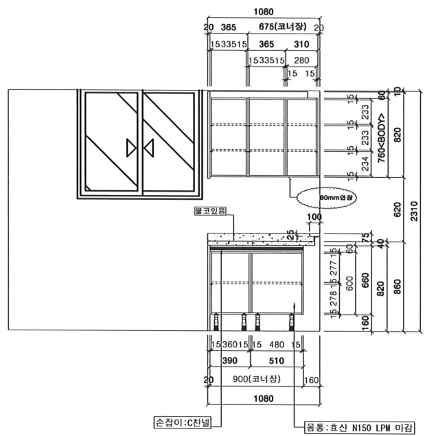
INNER VIEW-A
